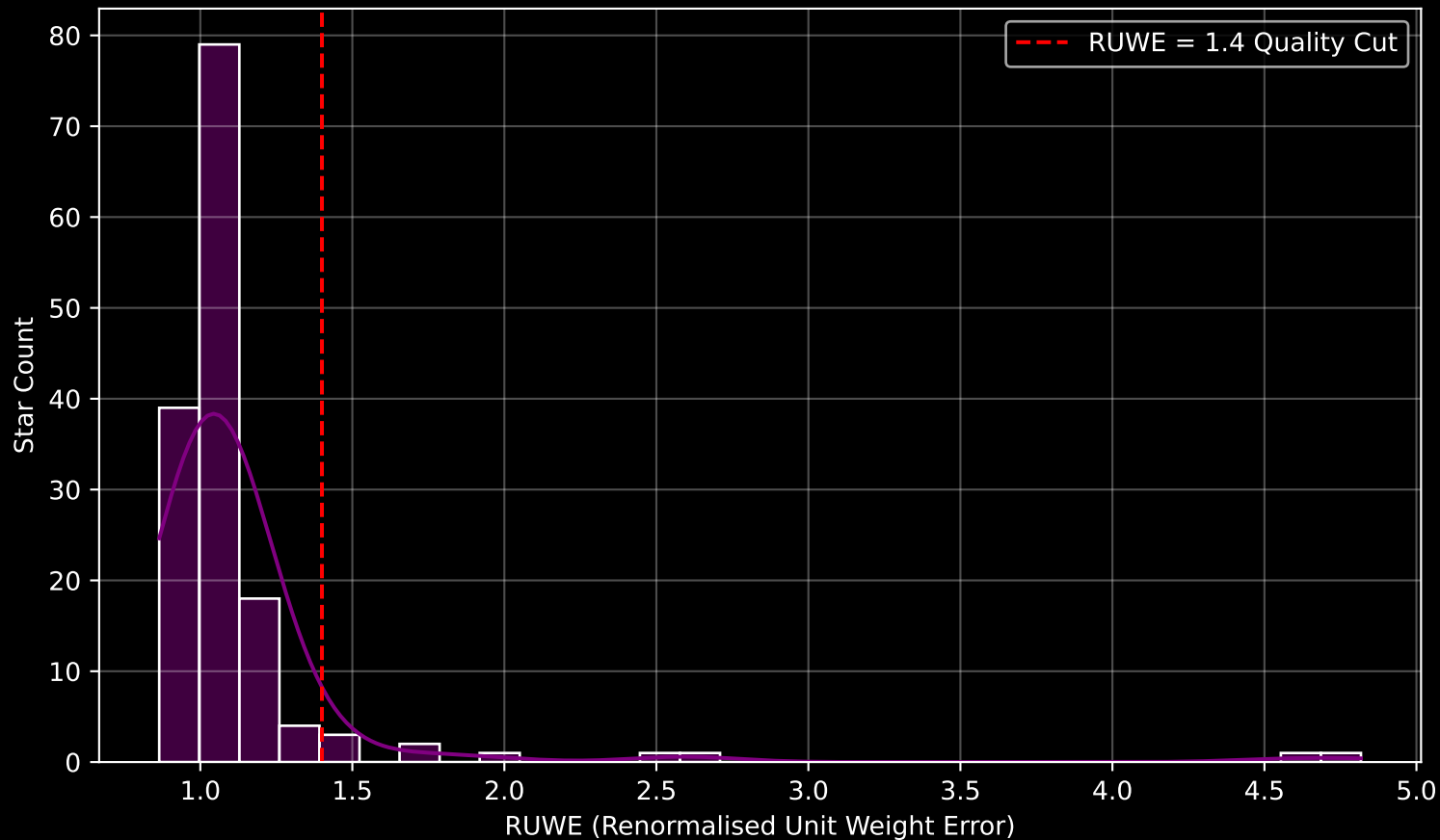
GAPOGEE DR17 Field [173+12] RUWE Distribution (n= 150)
