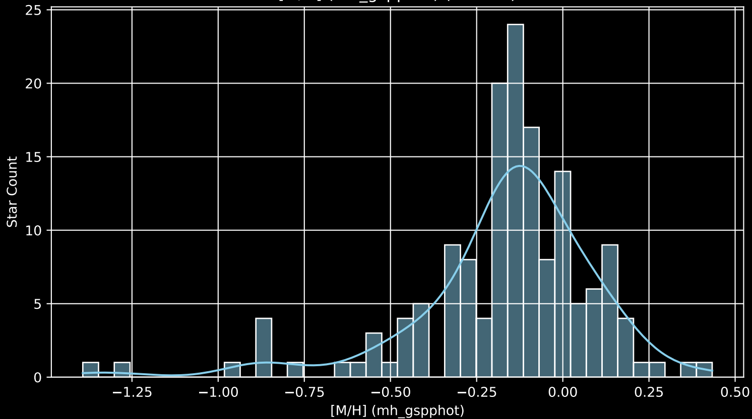
APOGEE DR17 Field: [173+12 [M/H] (mh_gspphot) (n= 155)
