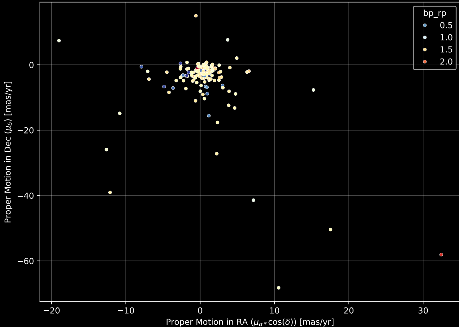
APOGEE DR17 Field: [173+12] Proper Motion Diagram (n= 156)
