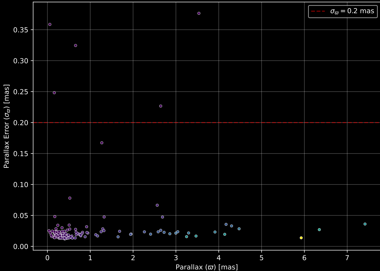
APOGEE DR17 Field: [173+12] Parallax Quality (n= 156)
