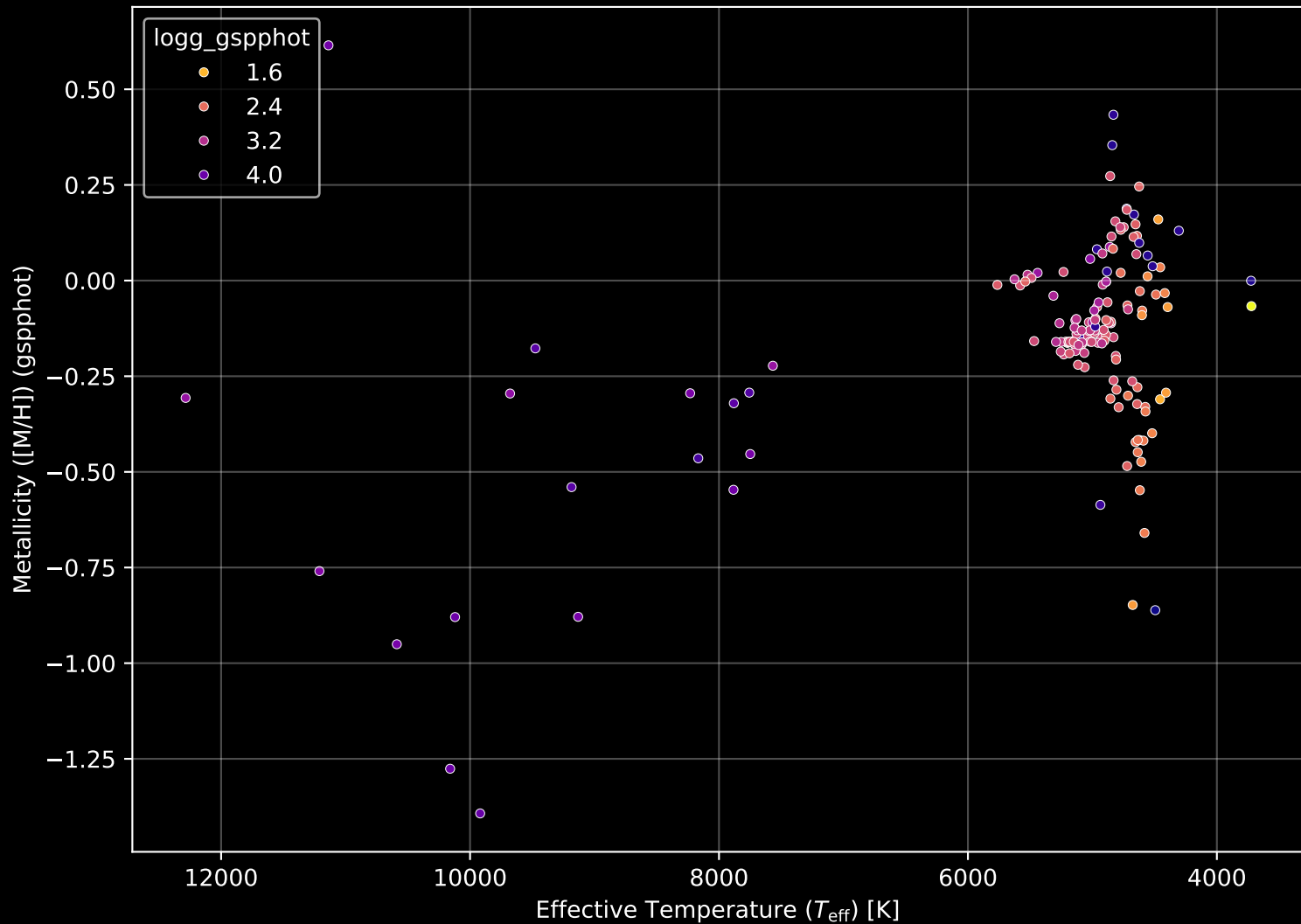
APOGEE DR17 Field: [173+12] Stellar Population Parameters (n= 156)
